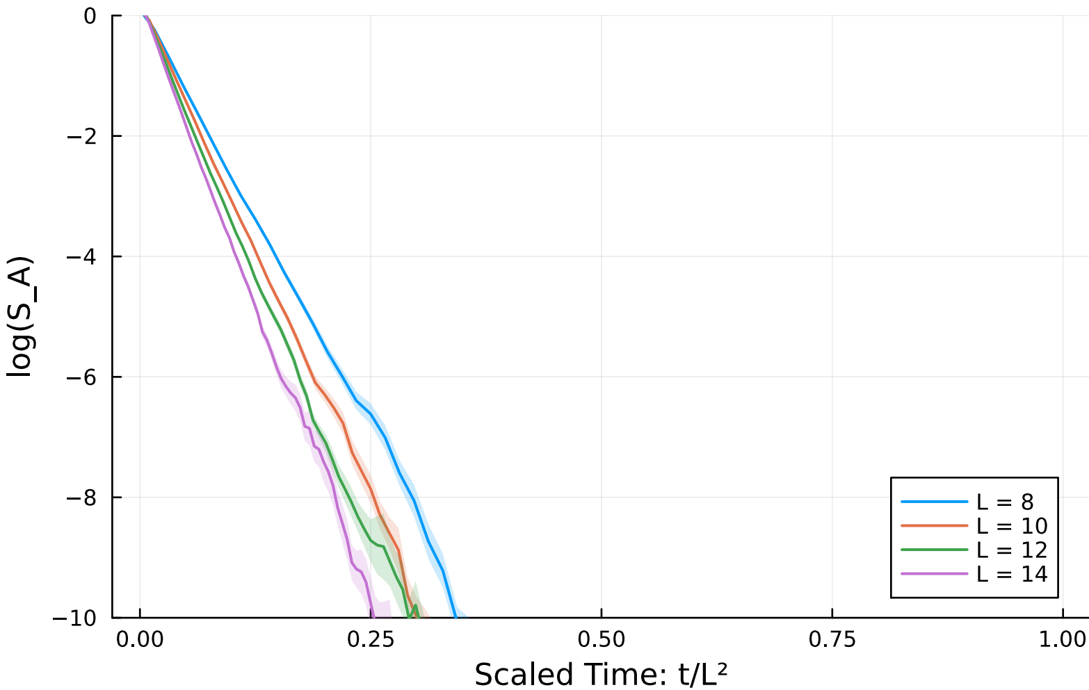
Scaled Log Entropy Evolution ( p = 0.616667 )
